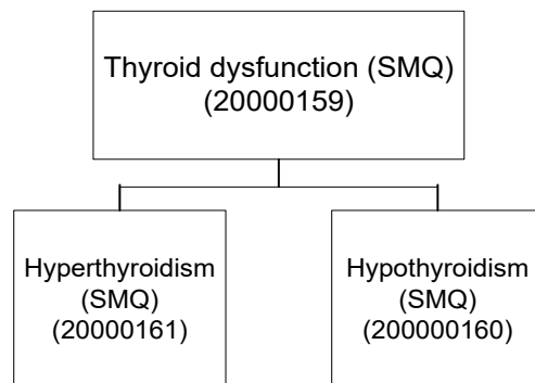
Figure 2-24. Hierarchy Structure of Thyroid dysfunction (SMQ)
